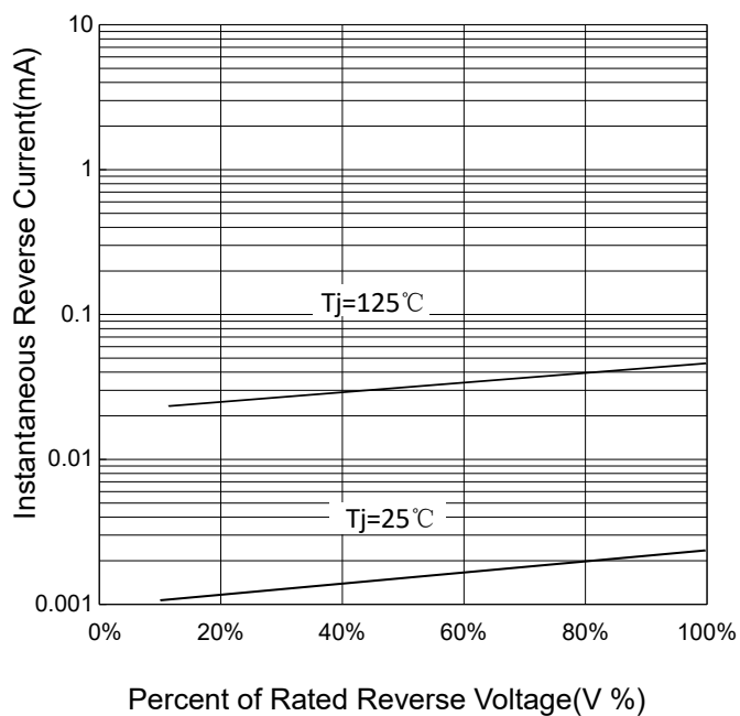
FIG 3: V R -I R
